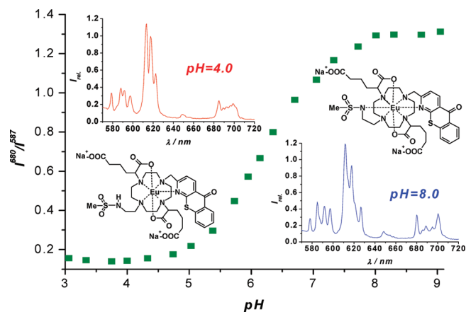
FIGURE 4. pH Dependence of the europium emission spectrum showing the two Eu(III) species ( \lambda_{exc} 380 nm, 298 K, 0.1 M NaCl).
